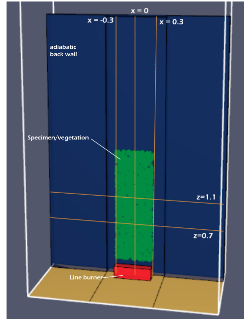
Figure 34: Calculations Lines Validation Study
