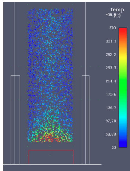
(b) Moisture content 50% - Particle Temperature at 350 sec
