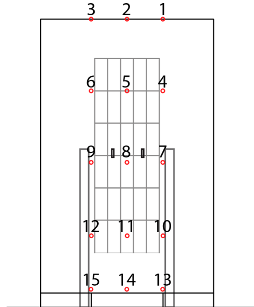
Figure 15: Numbering of thermocouples front view
