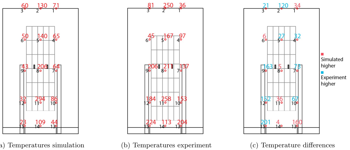
Figure 41: Maximum temperatures recorded per thermocouple
