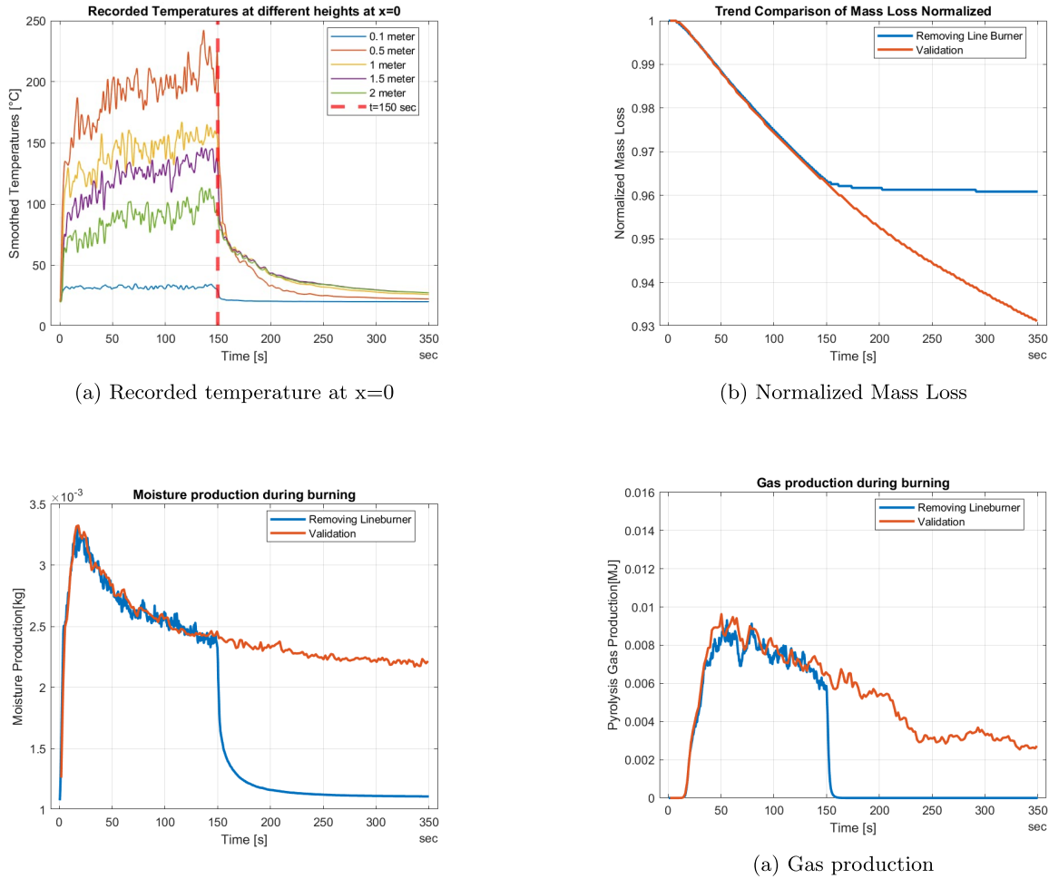
Figure 49: Different moisture Content Results
