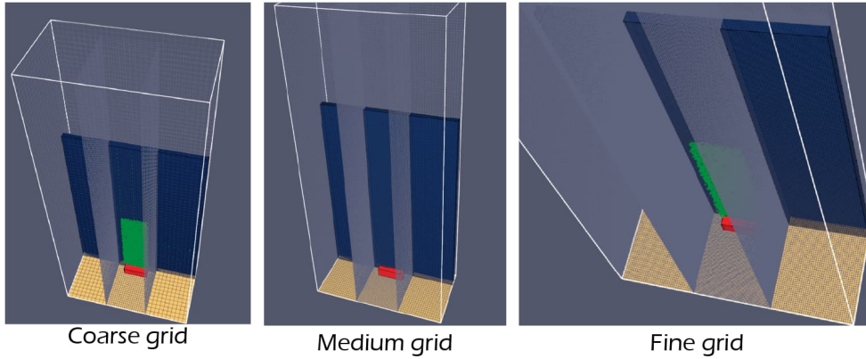
Figure 33: Grid levels
