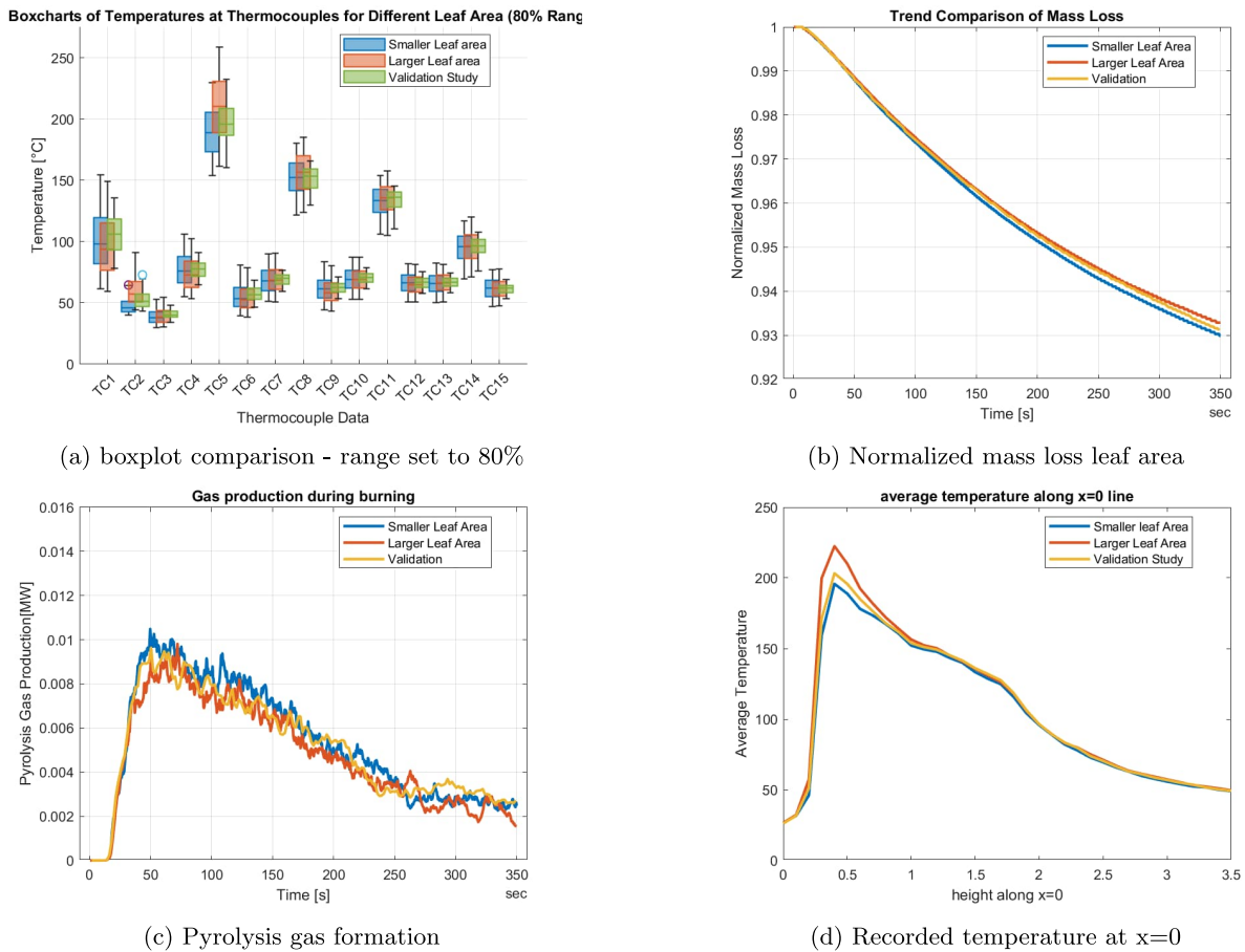
Figure 46: Results different leaf area simulation
