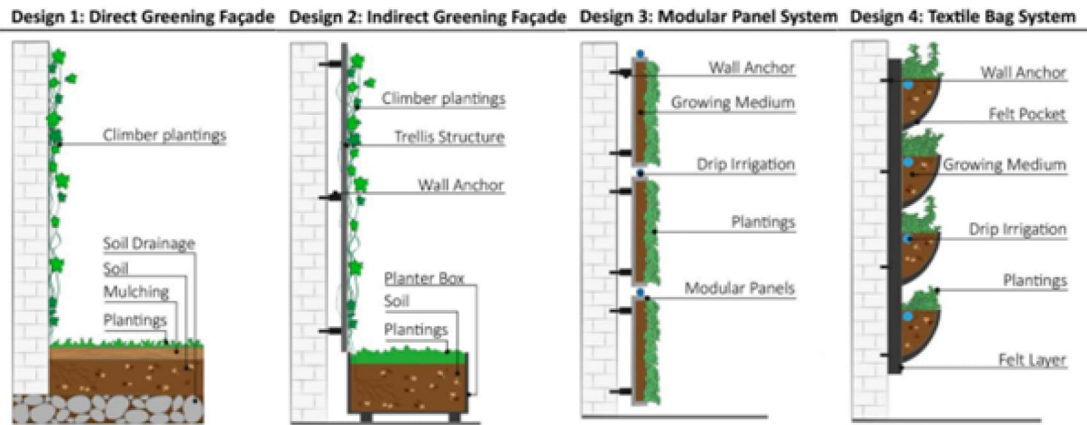
Figure 7: VGS types [4]
