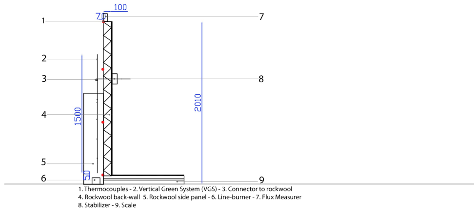
Figure 78: Setup 3
