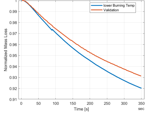
(b) Normalized mass loss burning temperature
